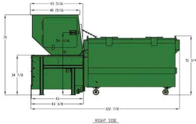
Typical Mini-M.A.C. Model 3A compactor configuration with chute system
