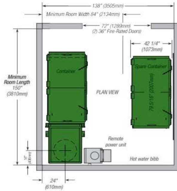
Typical Mini-M.A.C. Model 3A compactor configuration with chute system
